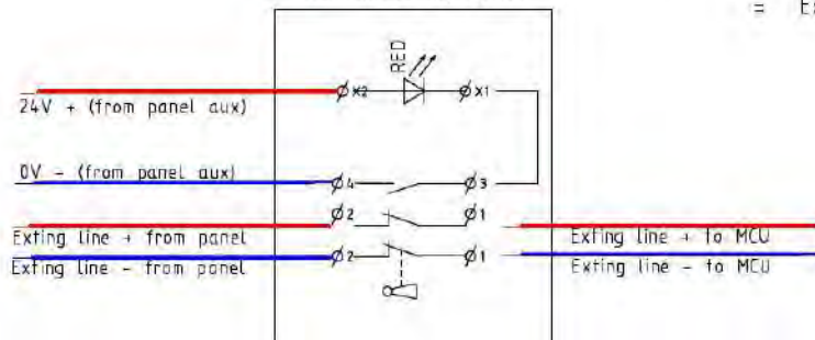
Maintenance Key switch
