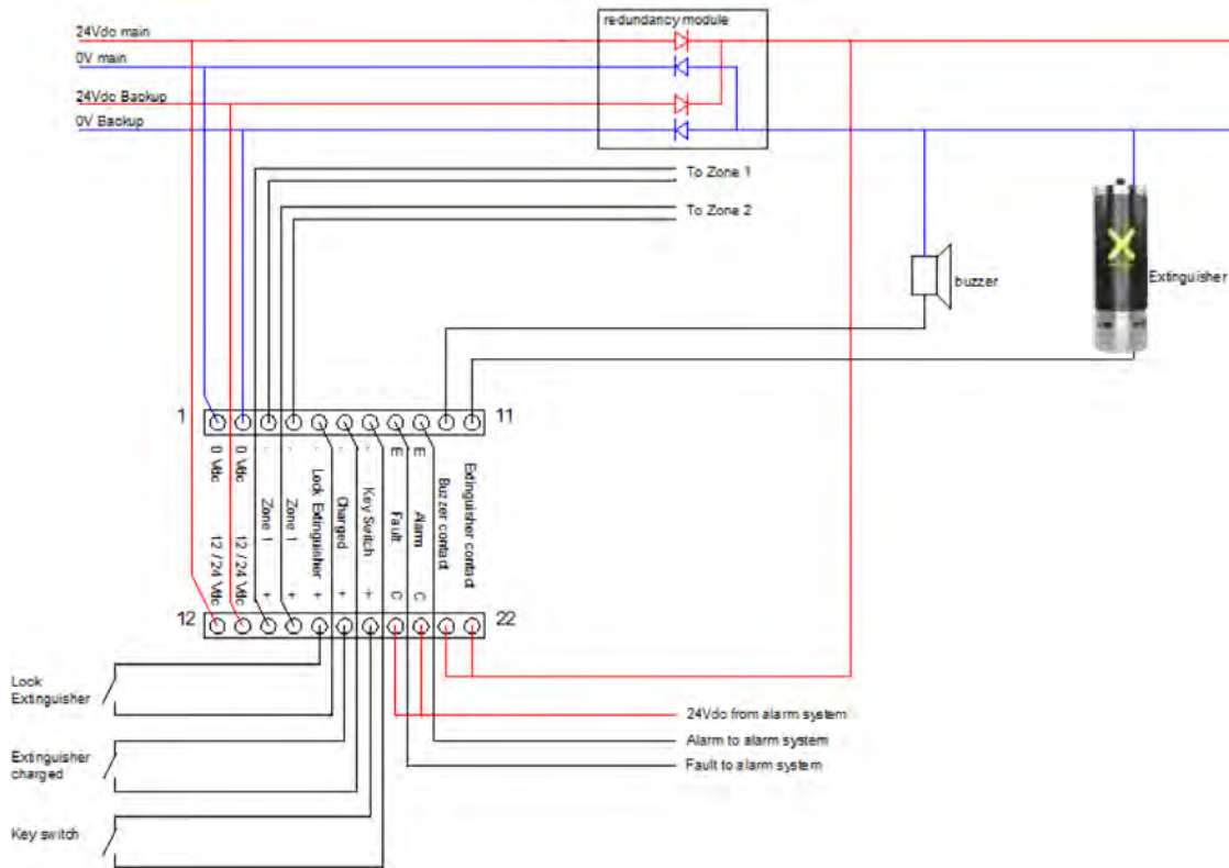
Installation schematic
