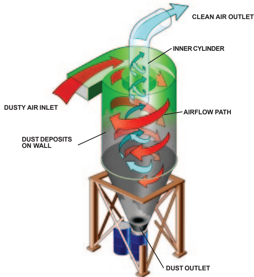
Figure 1: Cyclone Operation
