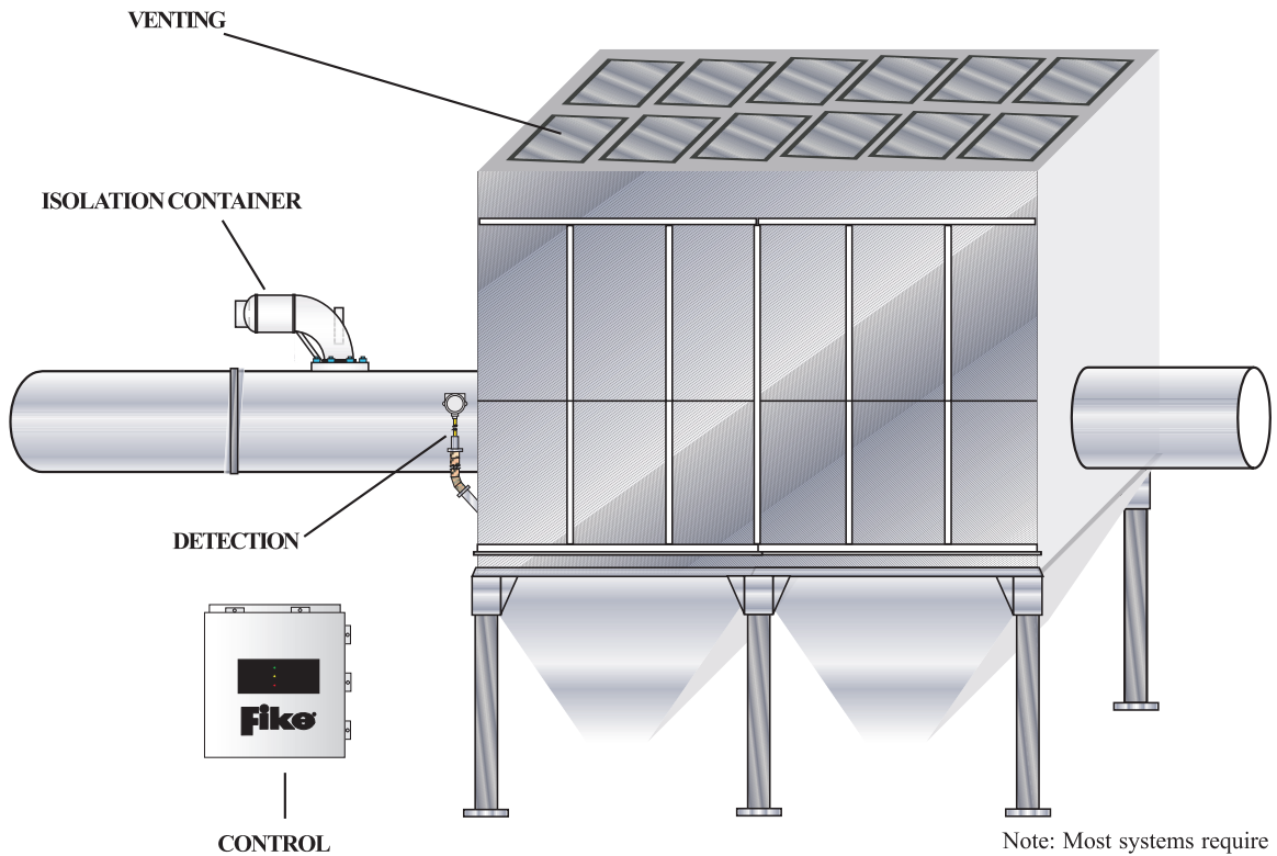
Figure 2: Electrostatic Precipitator Protected by Explosion Venting and Chemical Isolation
