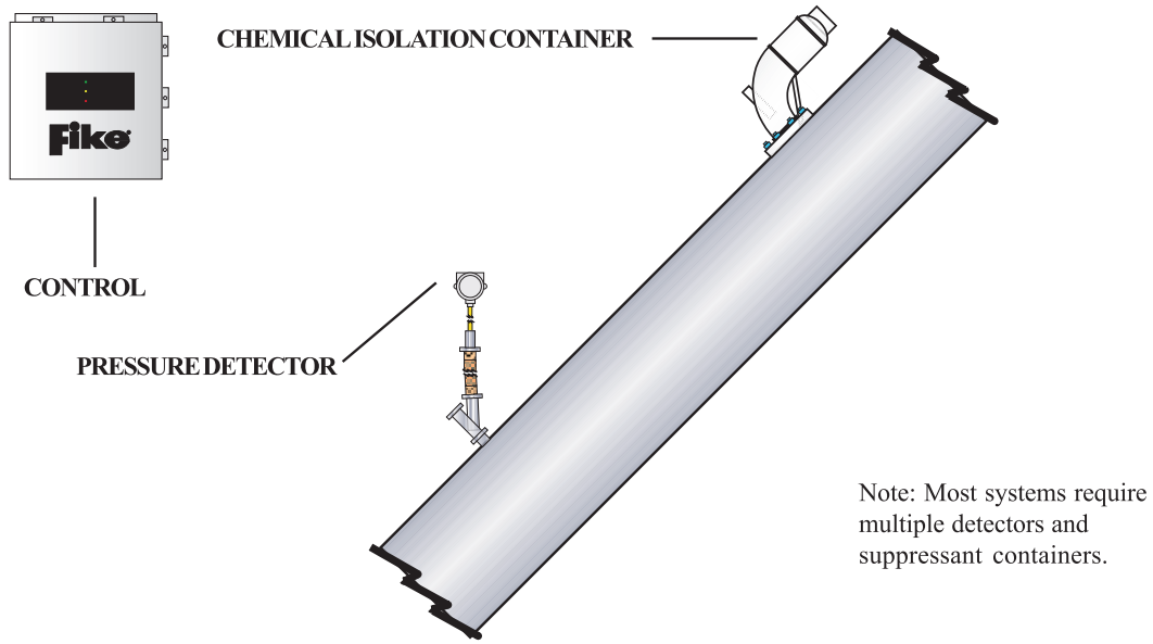
Figure 2: Transport Pipe Protected by Chemical Isolation
