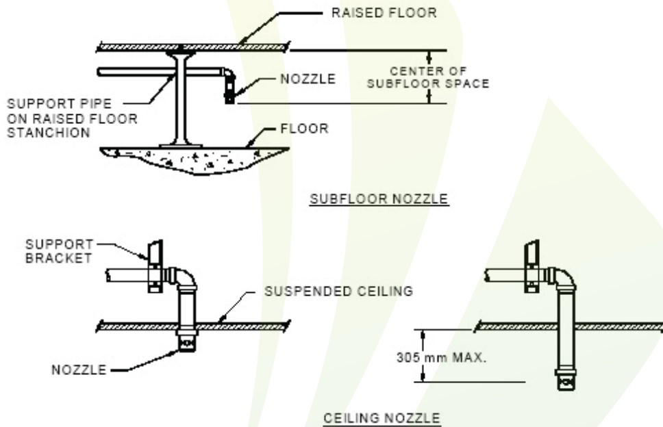
Nozzle Mounting Details
